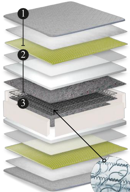
LFK 224 molas/m 2 arame bitola 2,2mm
